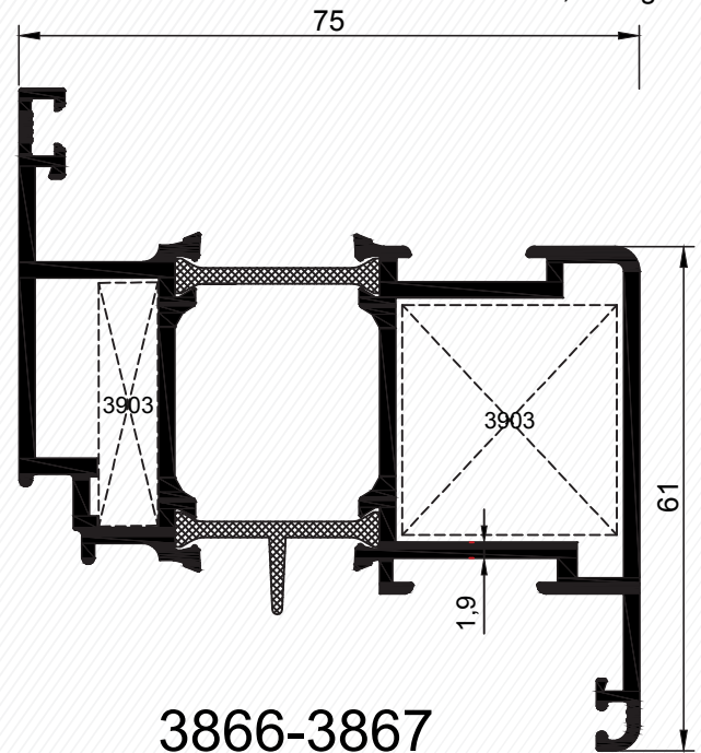
Geniş Kanat Profili - Large Sash Profile
