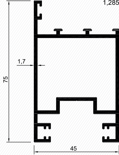
Kanat Profili - Sash Profile
