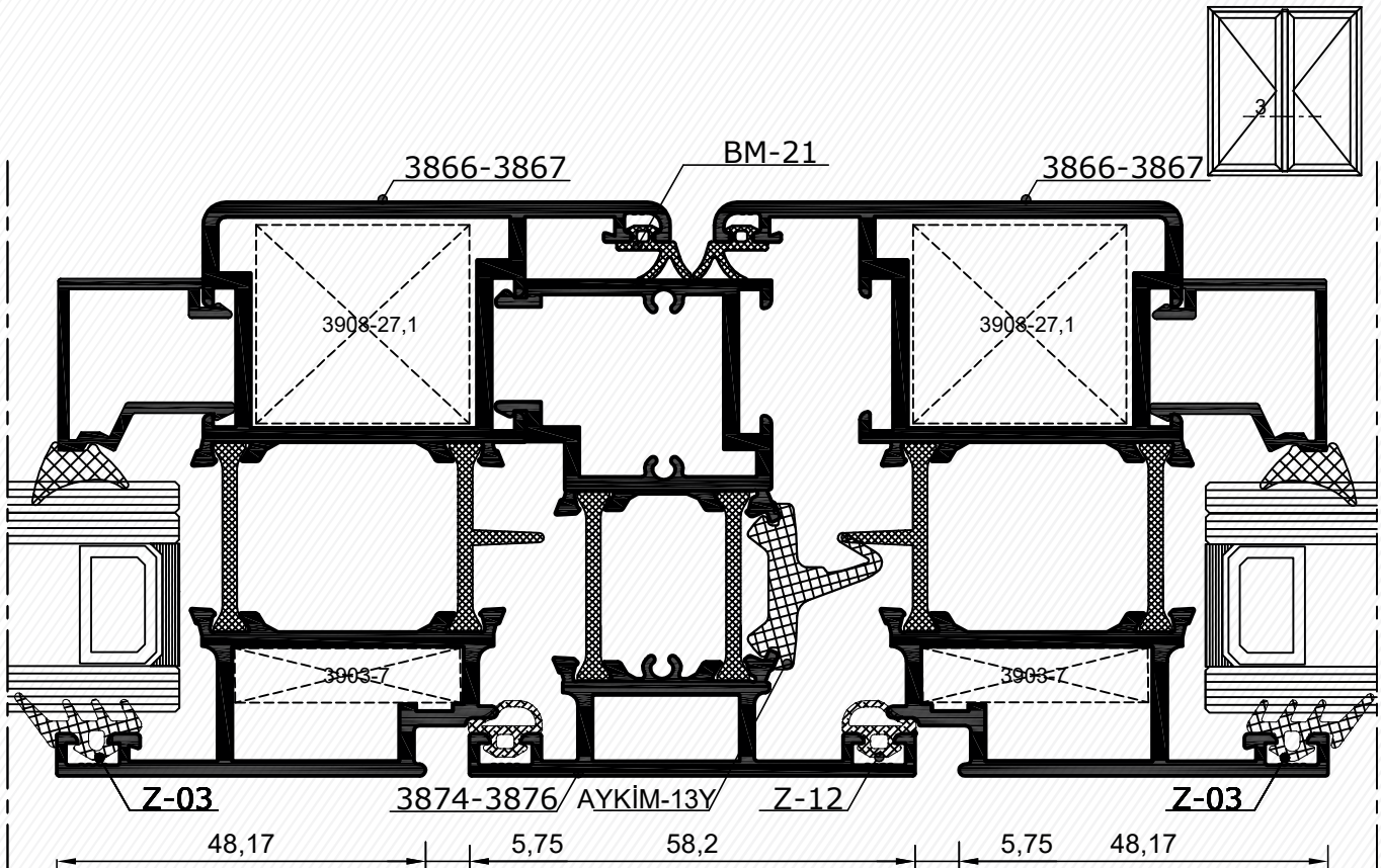
3 DETAYI DETAIL
