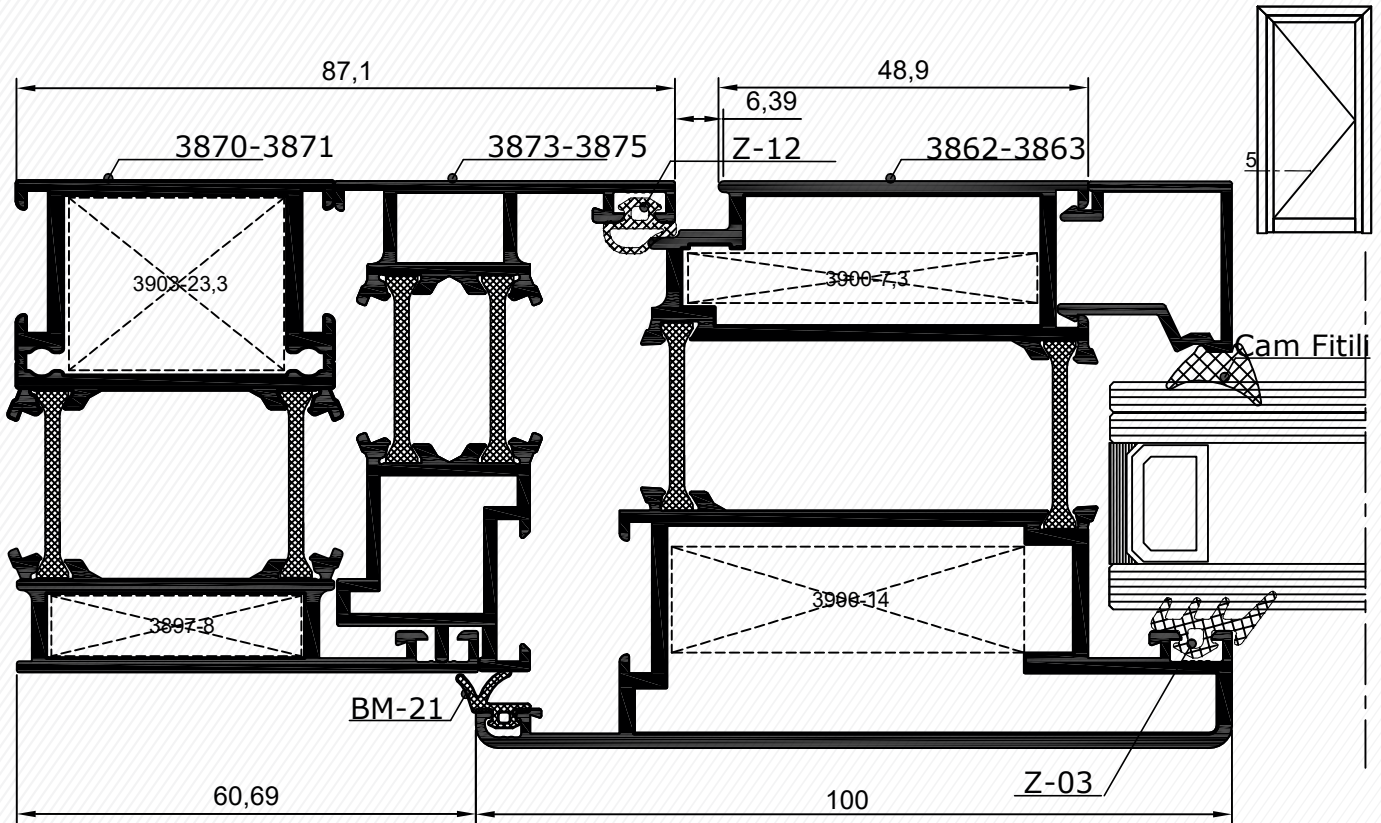
5 DETAYI DETAIL
