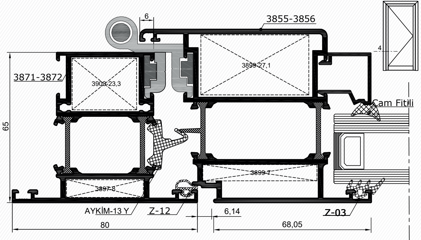
4 DETAYI DETAIL
