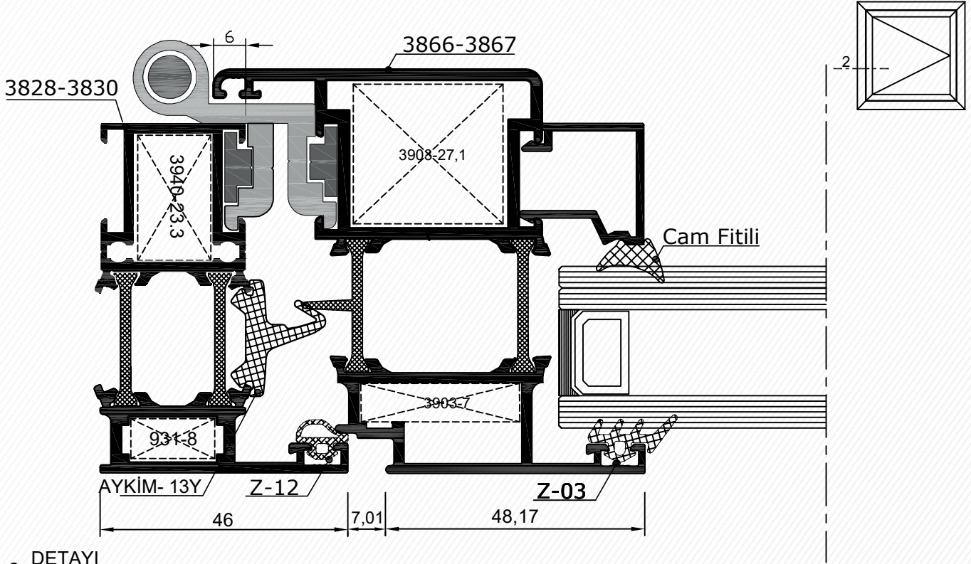
2 DETAYI DETAIL
