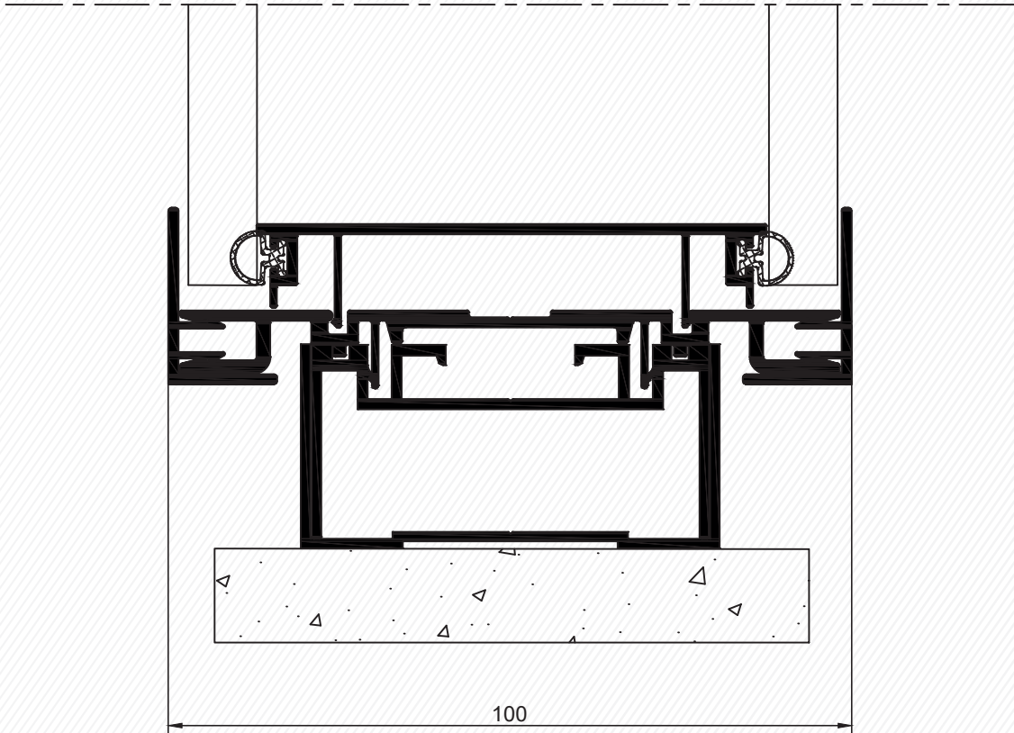
Sistem Kesiti System Section
