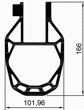
3739 9,931 kg/m
