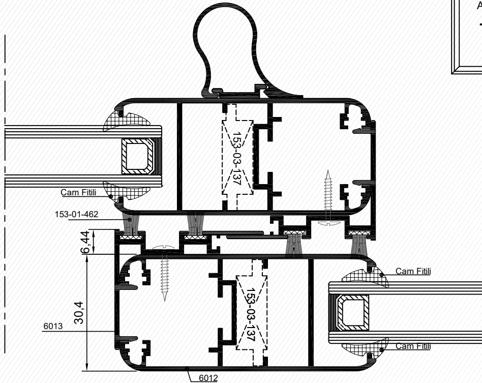
ALTERNATİF 2 DETAYI DETAIL
