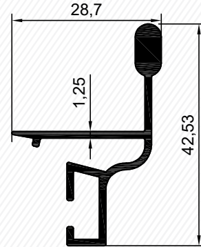
Sineklik Ray Profili Fly Screen Rail Profile
